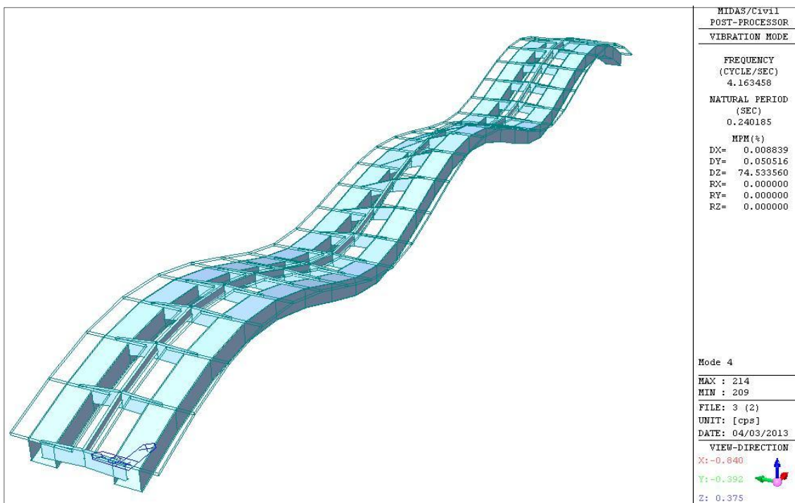
(b) Mode 4 ( f_4 = 4.1634 Hz )
