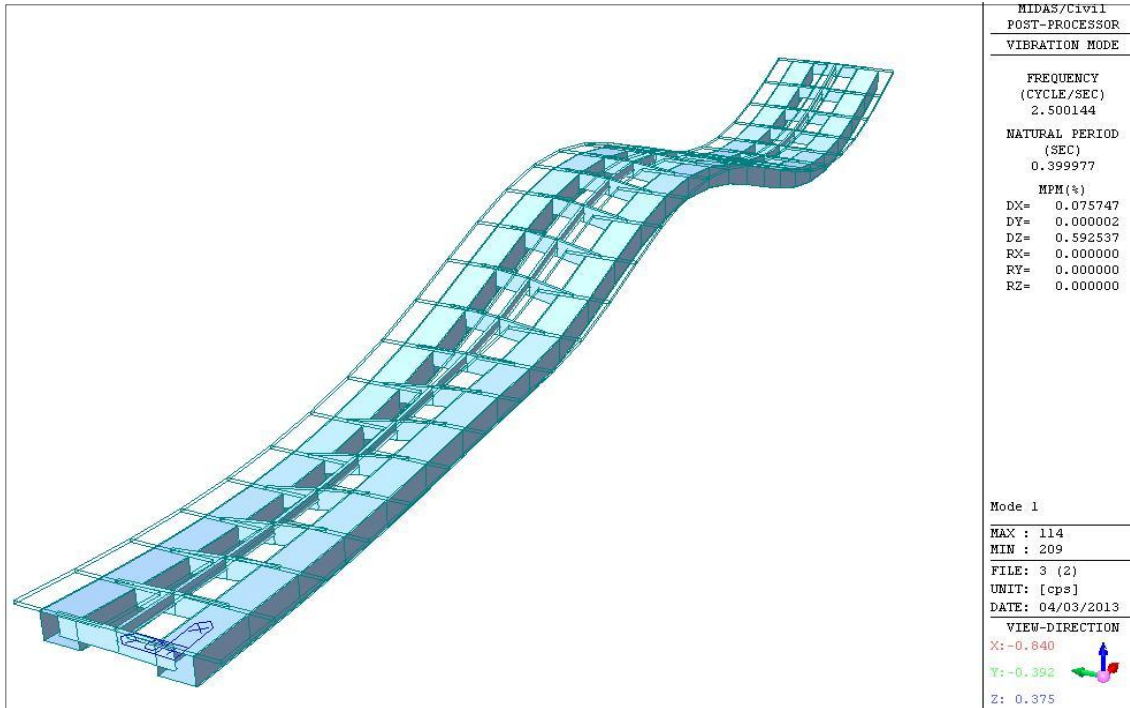
(a) Mode 1 ( f_1 = 2.5001 Hz )
