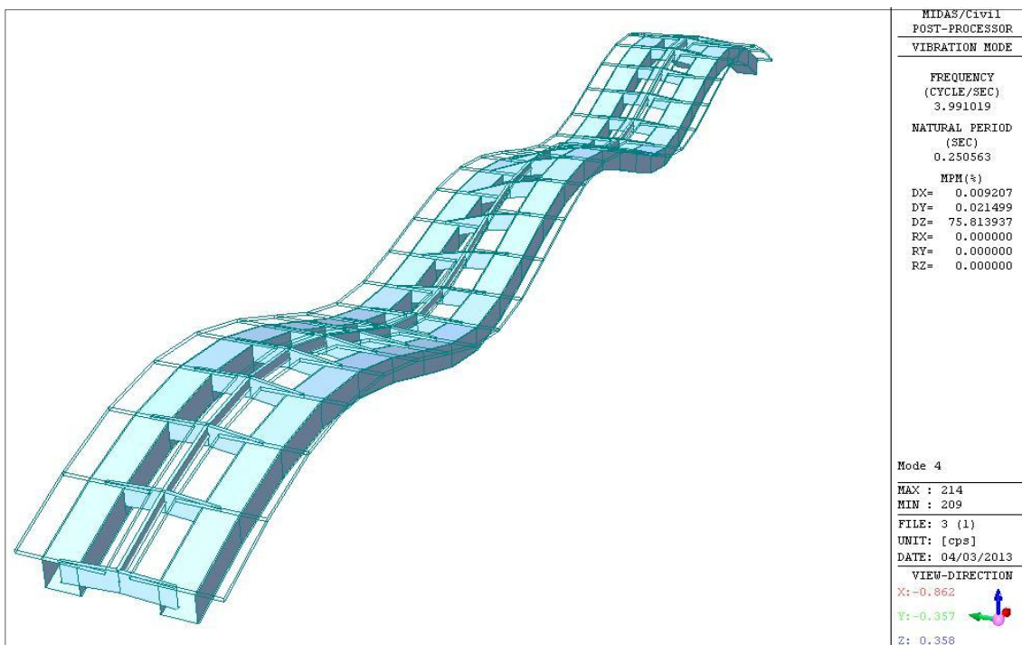
(b) Mode 4 ( f_4 = 3.9910 Hz )
