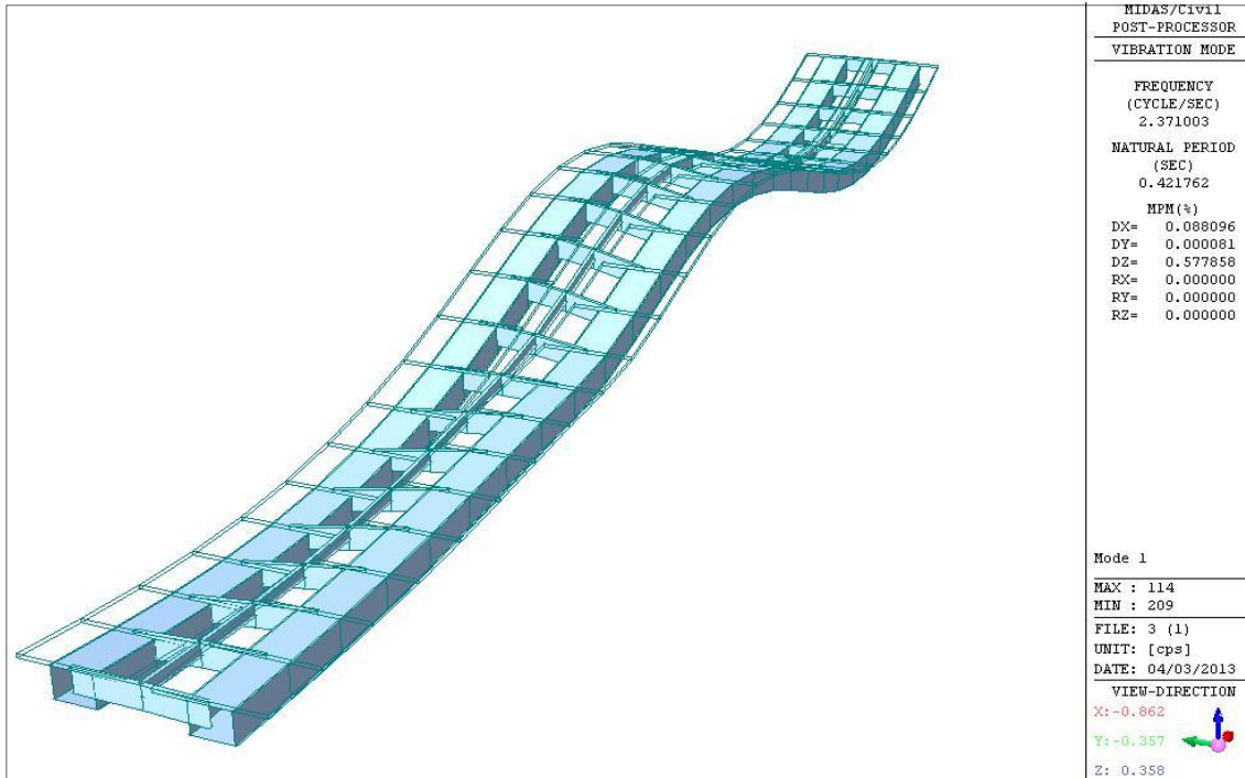
(a) Mode 1 ( f_1 = 2.3710 Hz )
